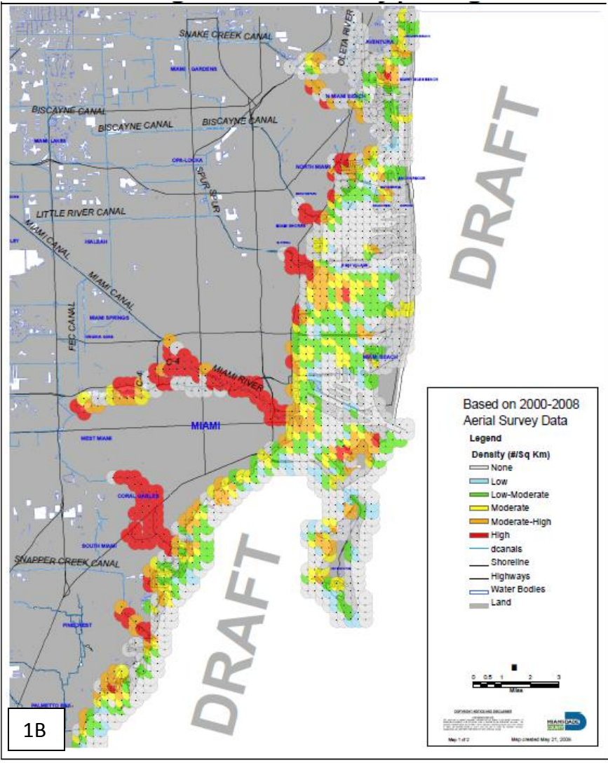
Figure 1A&B. GIS analysis of relative boat densities (Fig. 1A) (Gorzelany, 2009) and relative manatee densities (Fig. 1B) (DERM, 2009) in northern Biscayne Bay, using the Gorzelany (2009) method. Note the scale difference between the two due to the larger area covered by the DERM Manatee surveys. Also, the circles depicted in 1A are 1-mile radius, while circles in 1B are ¼-mile radius.
