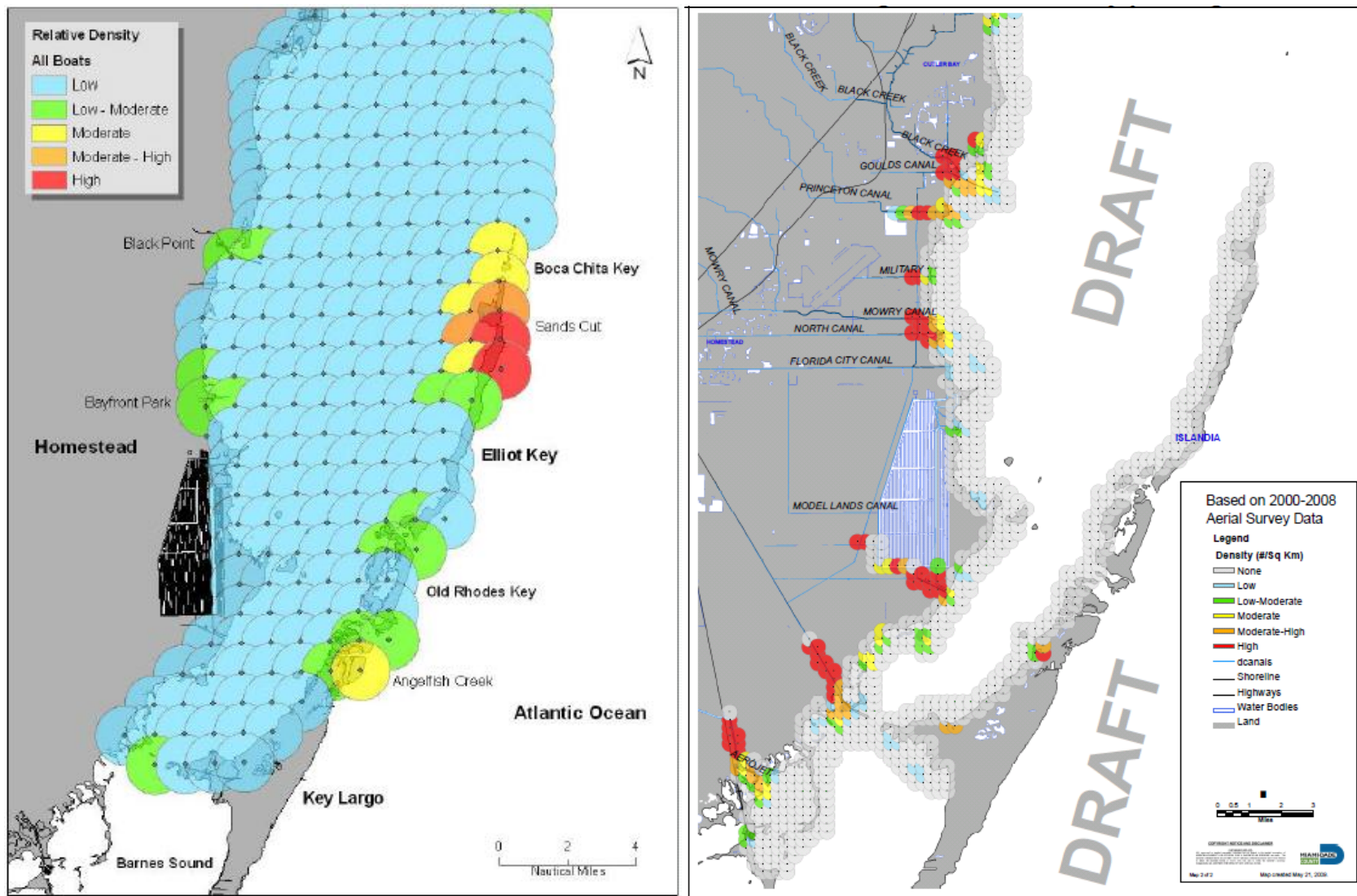
Figure 2A&B. GIS analysis of relative boat densities (Fig. 2A) (Gorzelany, 2009) and relative manatee densities (Fig. 2B) (DERM, 2009) in southern Biscayne Bay, using the Gorzelany (2009) method. Note the scale difference between the two due to the larger area covered by the DERM Manatee surveys. Also, the circles depicted in 1A are 1-mile radius, while circles in 1B are ¼-mile radius.
